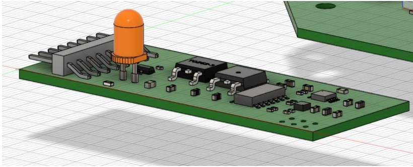
PCB 1 (Bottom)
