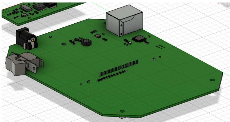
PCB 2 (Top)
