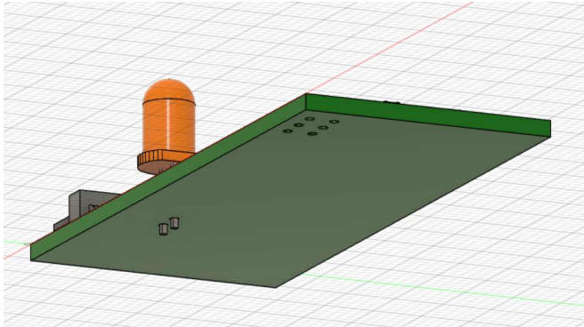
PCB 1 (Bottom)
